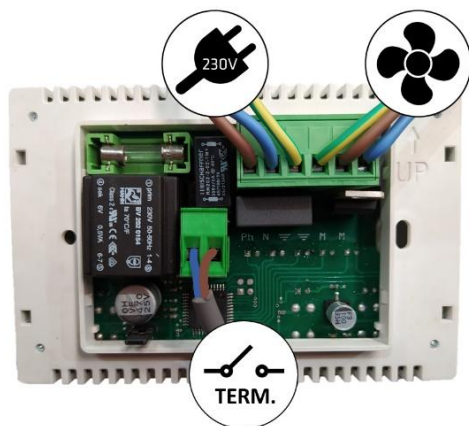
Figura n°18 - Potentiometeranschlüsse
