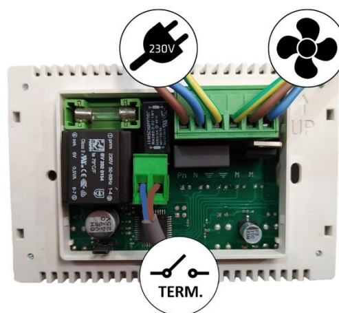
Potentiometeranschlüsse
