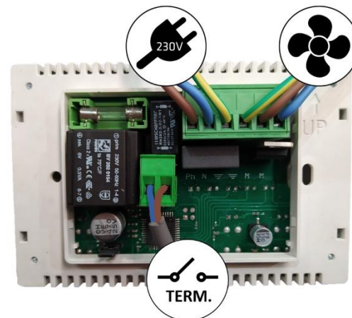
Potentiometeranschlüsse
