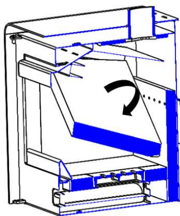
Figure No.10 - Extracting the vermiculite deflectors
