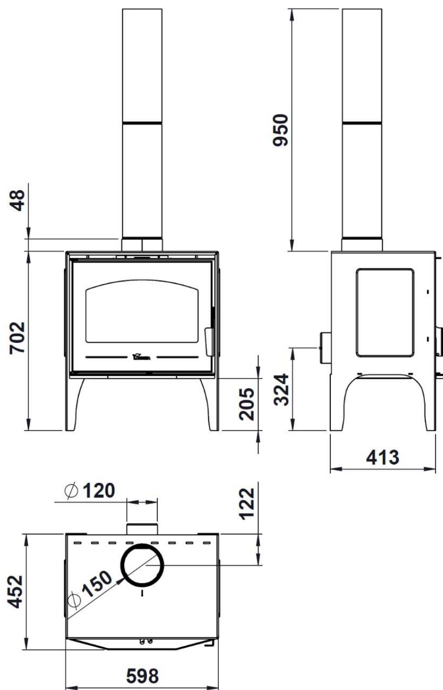
Figure No.1 - Dimensions of the CALPE series in mm
