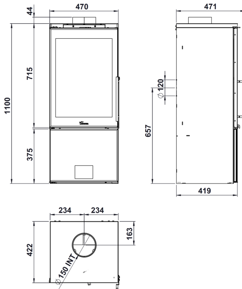
Figure No.1- Dimensions of the Dover
