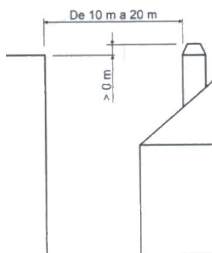
Figure No.16 - Distances between the chimney crown and objects within a radius of between 10 and 20m
