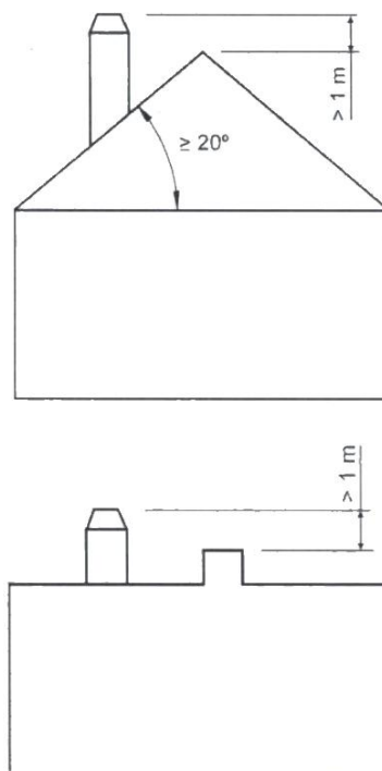
Figure No.14 - Distances between chimney crown and roof ridge
