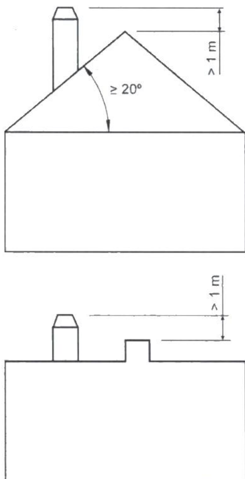
Figure No.6 - Distances between chimney crown and roof ridge
