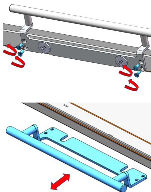
Figure No.45 - Screw removal and use as a cold handle handle
