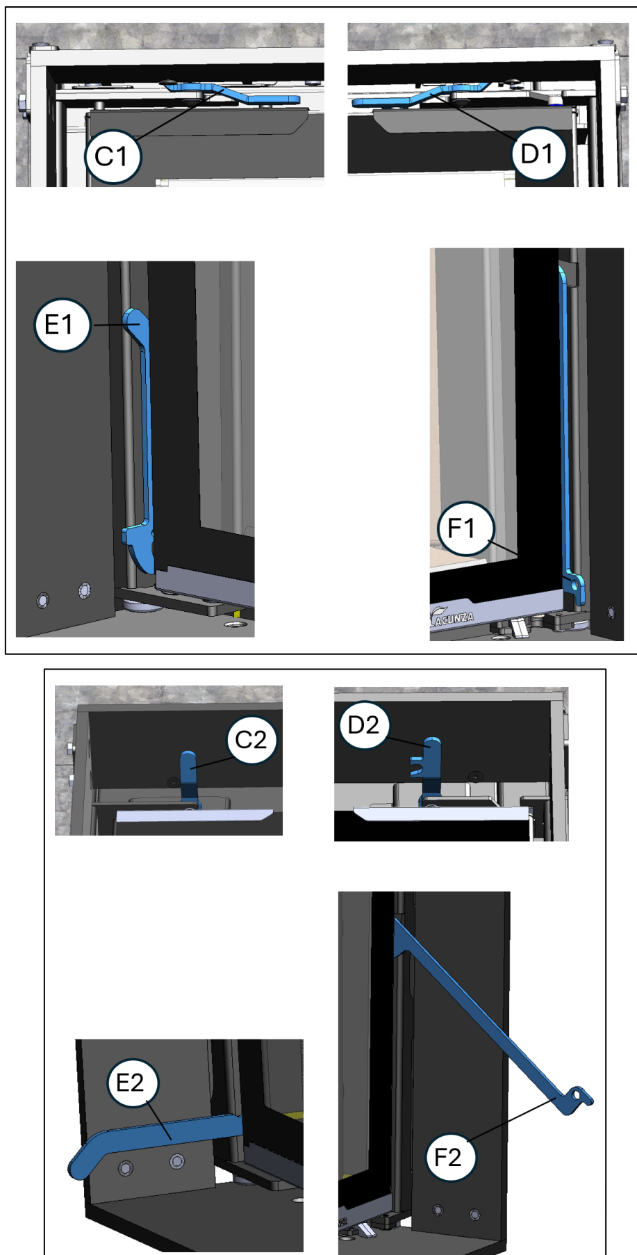
Figure No.27 - Operating components on the IZARO 60 CLI appliance
