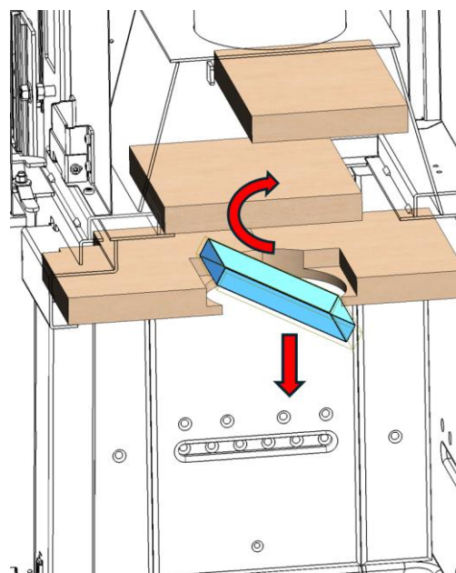
Figure No.31 - Removing the Izaro 60 CLI catalyst
