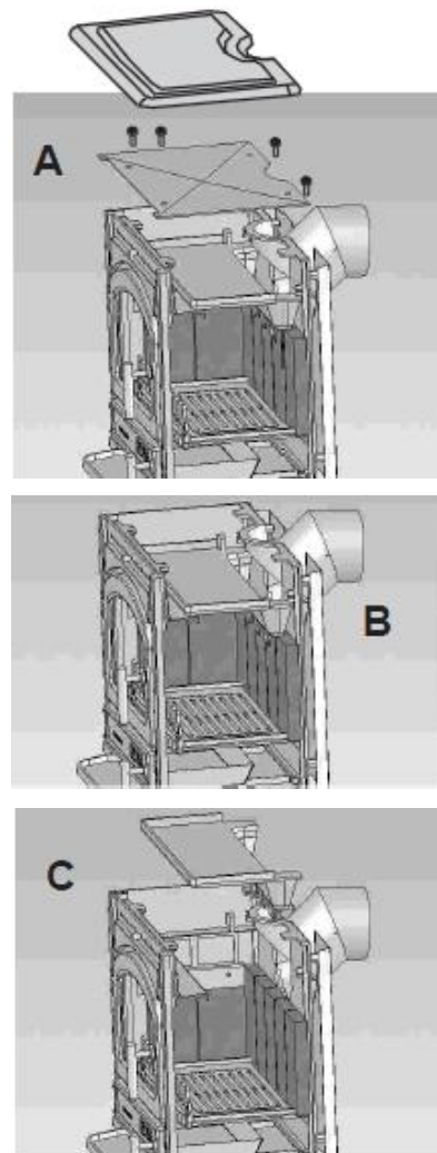
Figure No.9 - Removing the deflector
