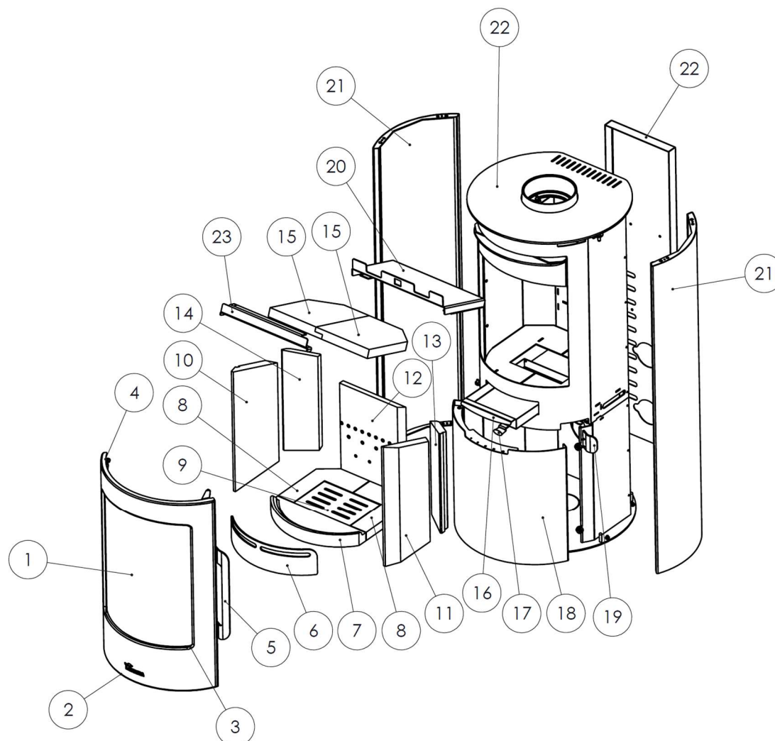
Figure No.1 - MAYA Exploded View
