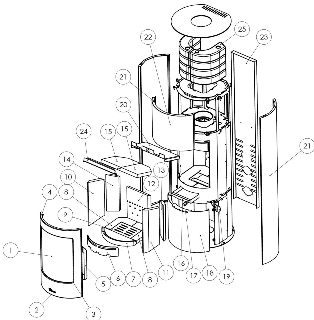
Figure No.3 - MAYA ACU Exploded View
