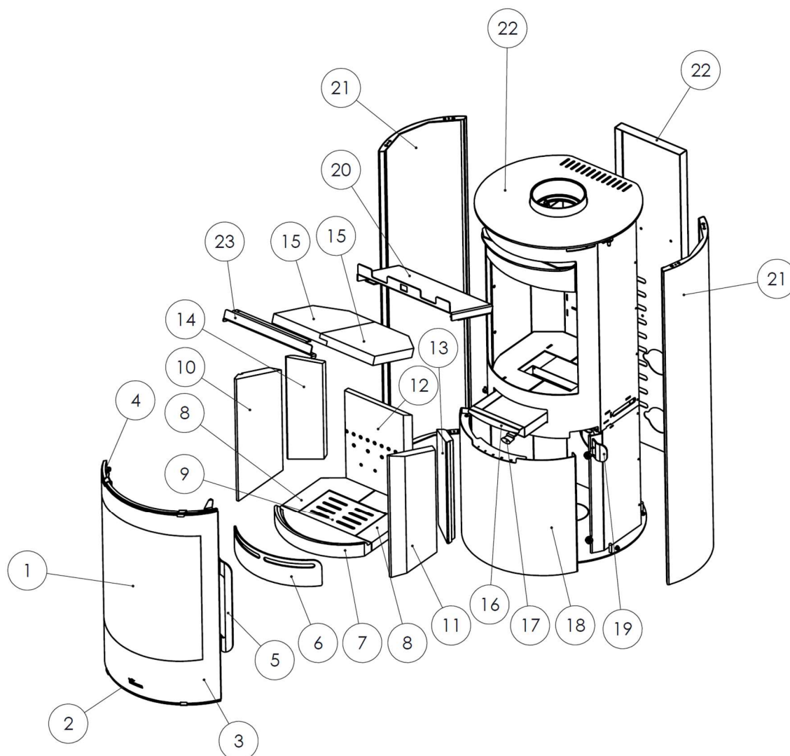
Figure No.2 - MAYA Vision Exploded View
