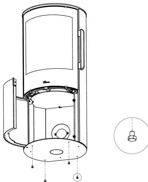
Figure No.19 - Installation of leveling feet
