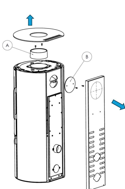
Figure No.5 - Interchange components (A) and (B) for rear smoke outlet
