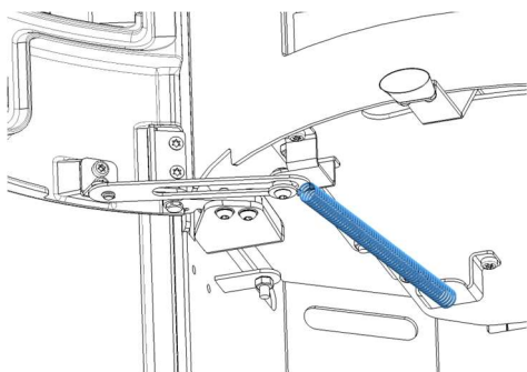
Figure No.20 - Step 1. Disassembling the spring
