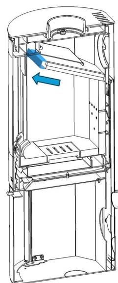
Figure No.16 - Removing the deflector
