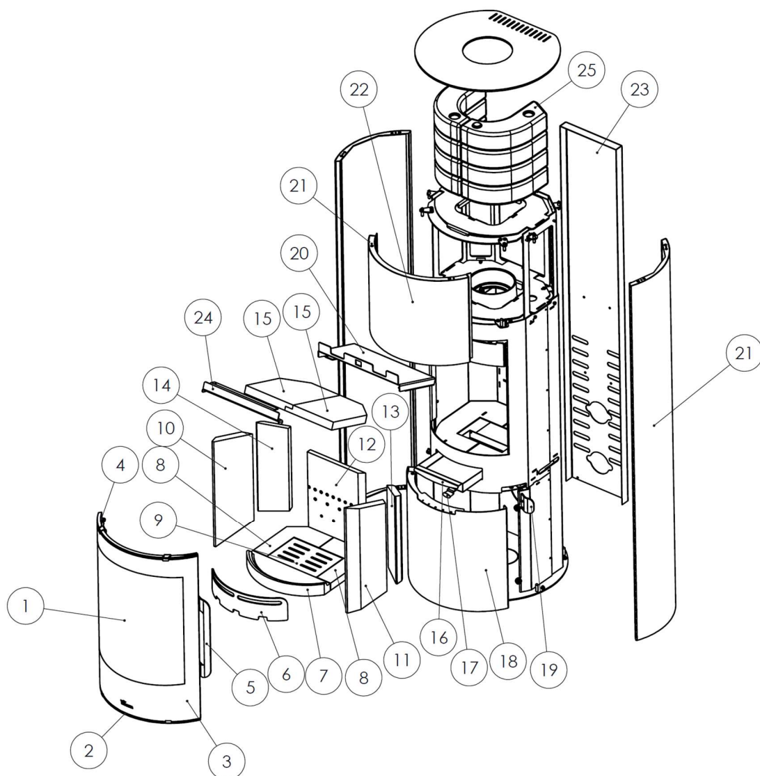
Figure No.4 - MAYA ACU Vision Exploded View
