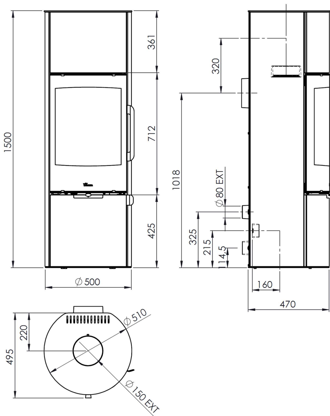
Figure No.2 - Dimensions of the MAYA ACU and MAYA ACU Vision appliance in mm
