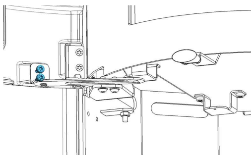
Figure No.22 - Step 3. Remove door support screws
