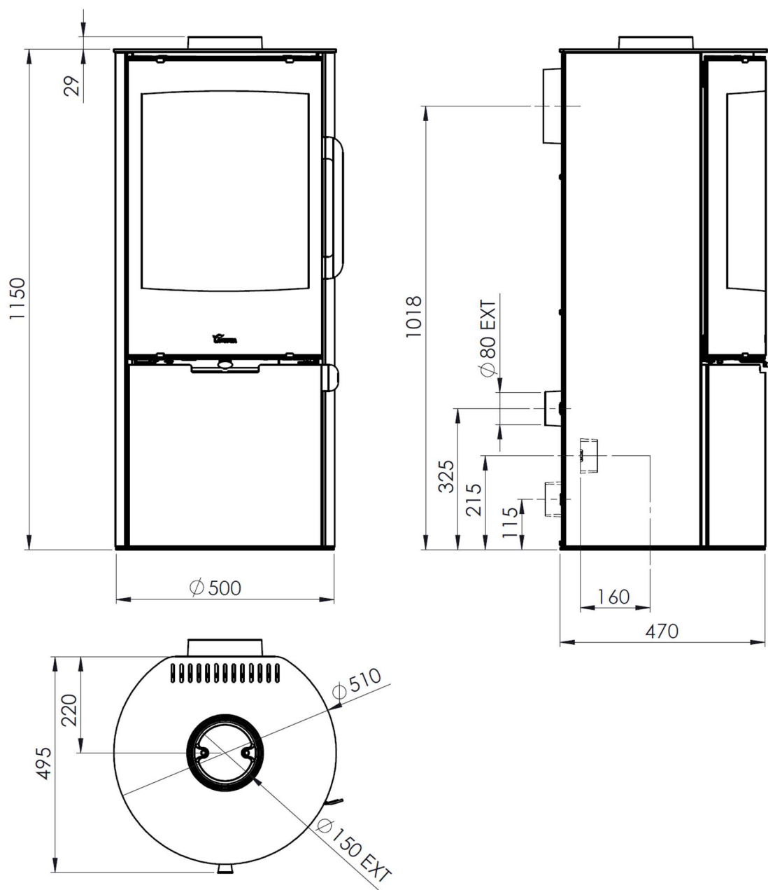
Figure No.1 - Dimensions of the MAYA and MAYA Vision appliance in mm
