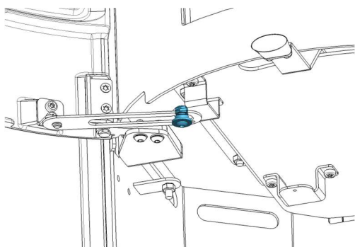
Figure No.20 - Step 1. Disassembling the spring
