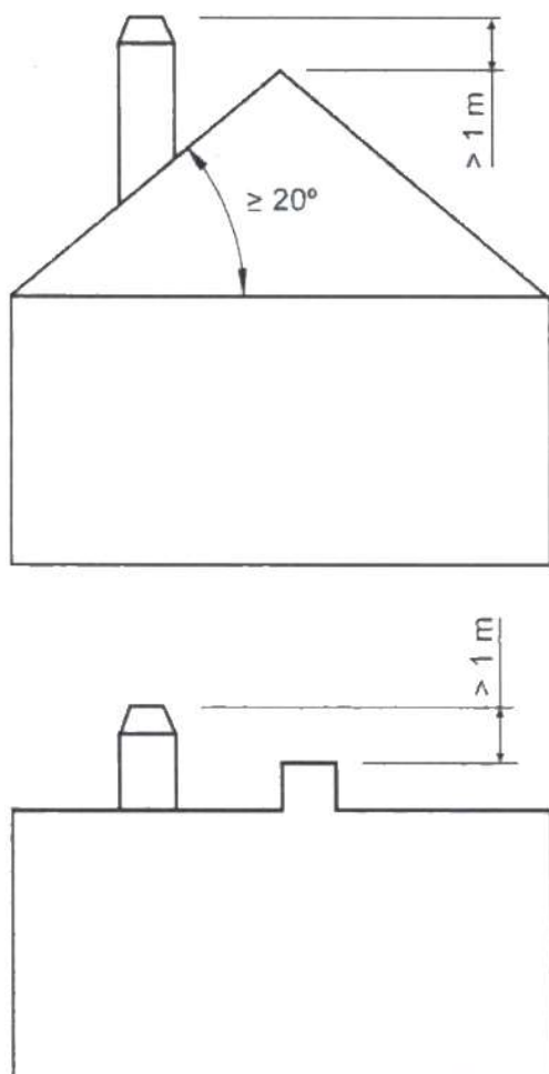
Figure No.10 - Distances between chimney crown and roof ridge
