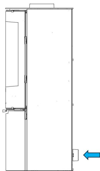
Figure No.7 - OPTION 1 (Installed) Air conduction for the combustion chamber
