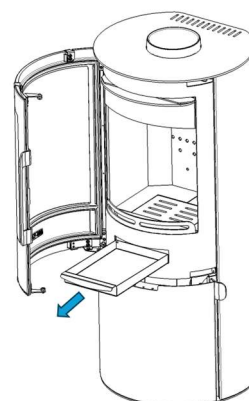
Figure No.15 - Removal of the ashtray
