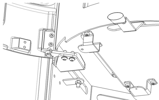
Figure No.23 - Step 4. Remove mechanism
