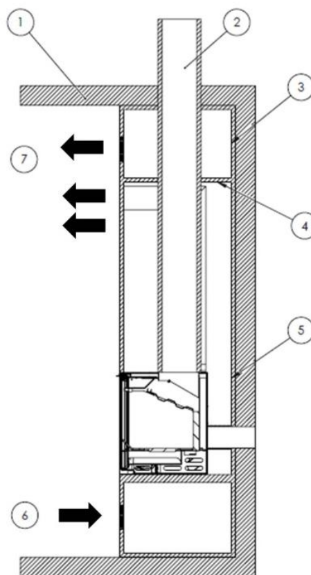
Figure No.7 - Interior diagram of the casing
