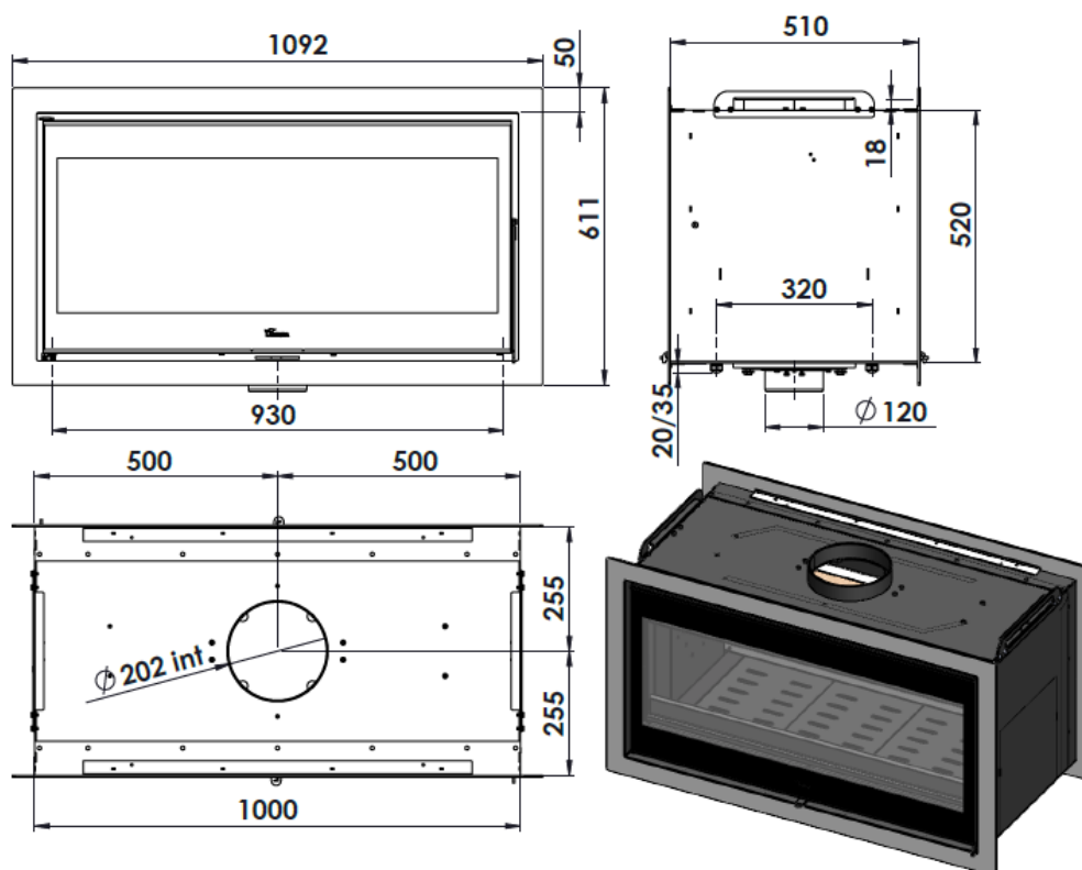
Figure No.3 - Dimensions of the Nickel 1000 appliance in mm
