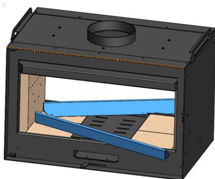
Figure No.17 - Removing the two Nickel separators.
