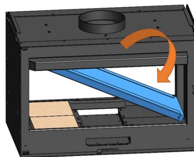
Figure No.21 - Drop the refractory holding it
