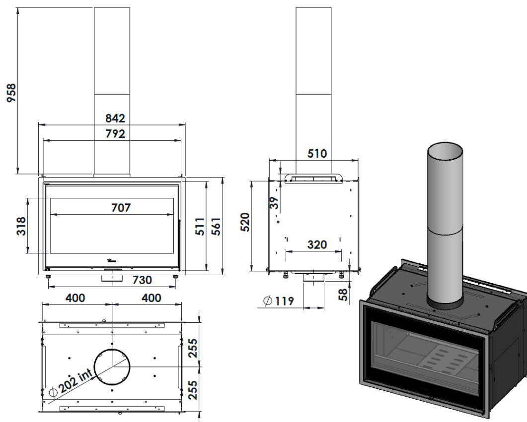
Figure No.2 - Dimensions of the Nickel 800 appliance in mm
