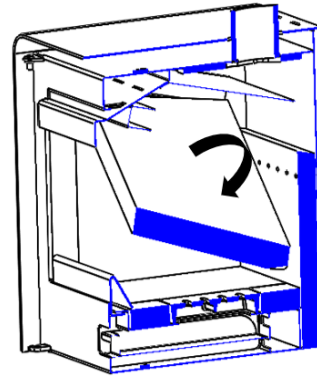
Figure No.15 - Extracting the vermiculite deflectors
