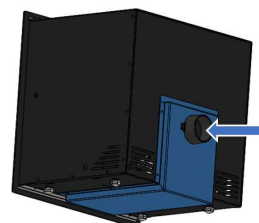
Figure No.13 - Accessory to channel the air inlet from the rear
