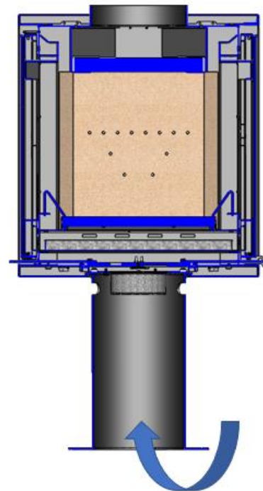
Figure No.7 - Piping air to the firebox in Verona 801-1001
